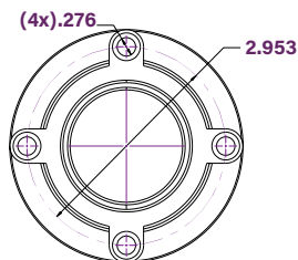
Output Cover
