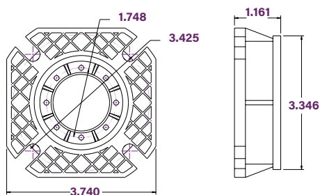
Output Flange
