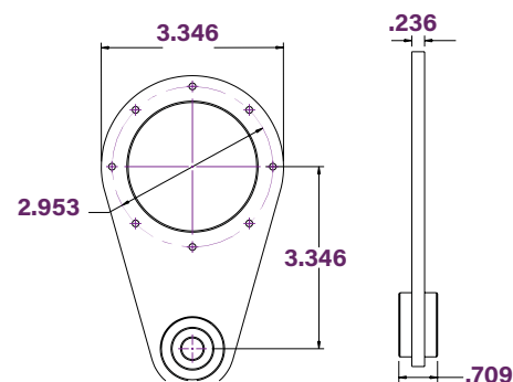
Torque Arm
