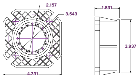
Output Flange
