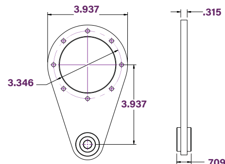
Torque Arm
