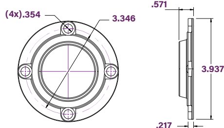
Output Cover
