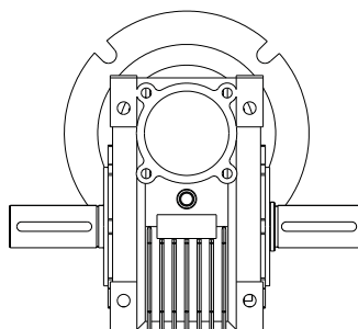
VMRV-63 with OSD
