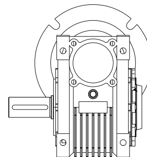
VMRV-63 with OSS & CVR
