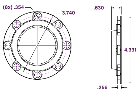
Output Cover
