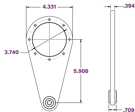
Torque Arm
