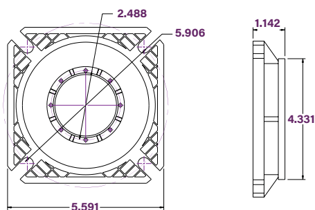
Output Flange
